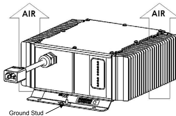
Figure 1: Charger Mounting
